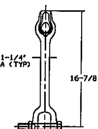
THIMBLE EYE ADAPTER T110-0311 (GALV)
