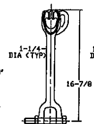
TRIPLE EYE ADAPTER T110-0465 (GALV)
