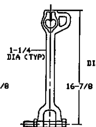
TWINEYE ADAPTER T110-0964 (GALV)
